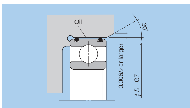
Fig. 4. Design of housing
