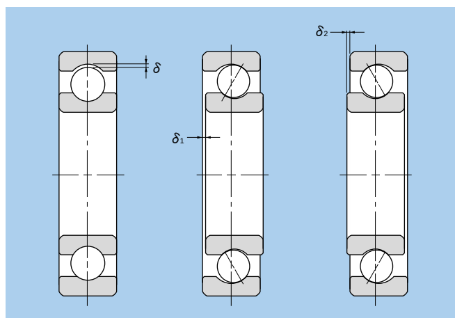
Fig. 8.1 Internal clearance
