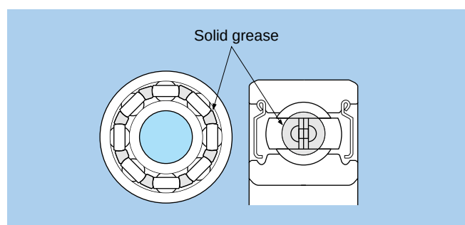
Fig. 11.3 Deep groove ball bearing with spot-pack solid grease (Z shield) (Standard for deep groove ball bearings)
