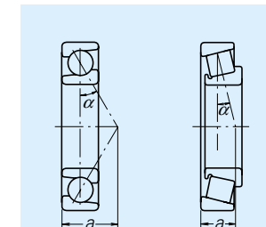
Fig. 5.11 Effective Load Centers
