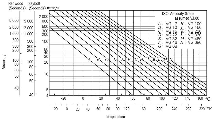
Fig. 12.11 Temperature-Viscosity Chart
