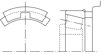
Fig. 14.11 Removal Notches
