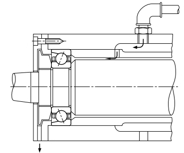
Fig. 12.9 Oil Mist Lubrication
