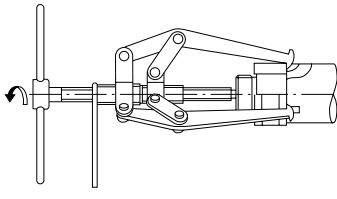
Fig. 14.14 Removal of Inner Ring Using Withdrawal Tool (2)
