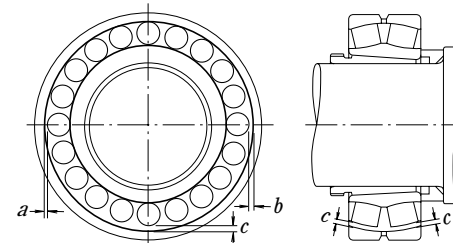
Fig. 14.9 Measuring Clearance in Large Spherical Roller Bearing
