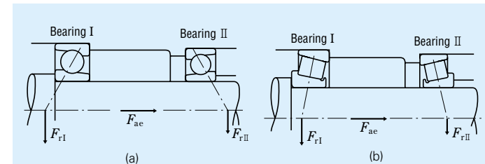
Fig. 5.12 Loads in Opposed Duplex Arrangement
