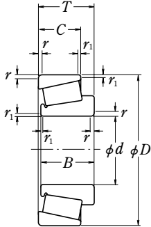
Fig. 7.2 Tapered Roller Bearings
