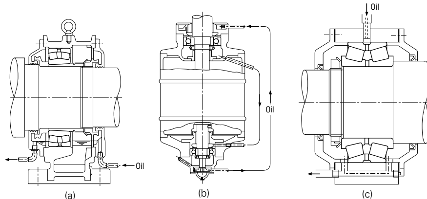
Fig. 12.7 Circulating Lubrication
