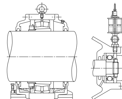
Fig. 12.5 Drip Feed Lubrication
