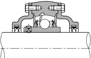
Fig. 2.3 Cast iron cover
