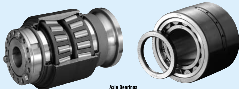
Axle Bearings
