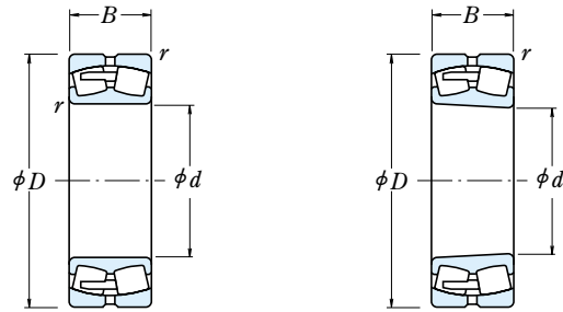
Cylindrical Bore
