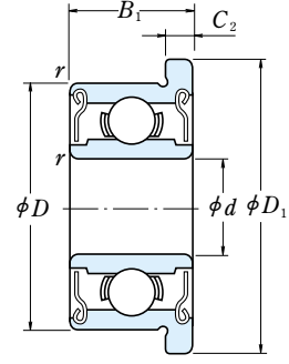
Shielded Type ZZ · ZZS
